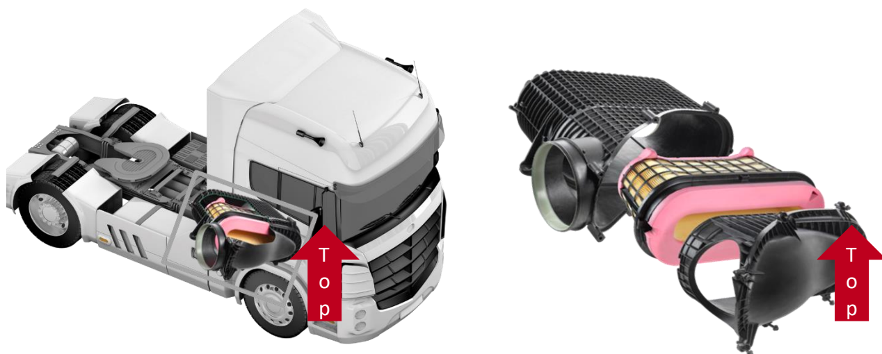
Mounting situation on the vehicle and in the housing
