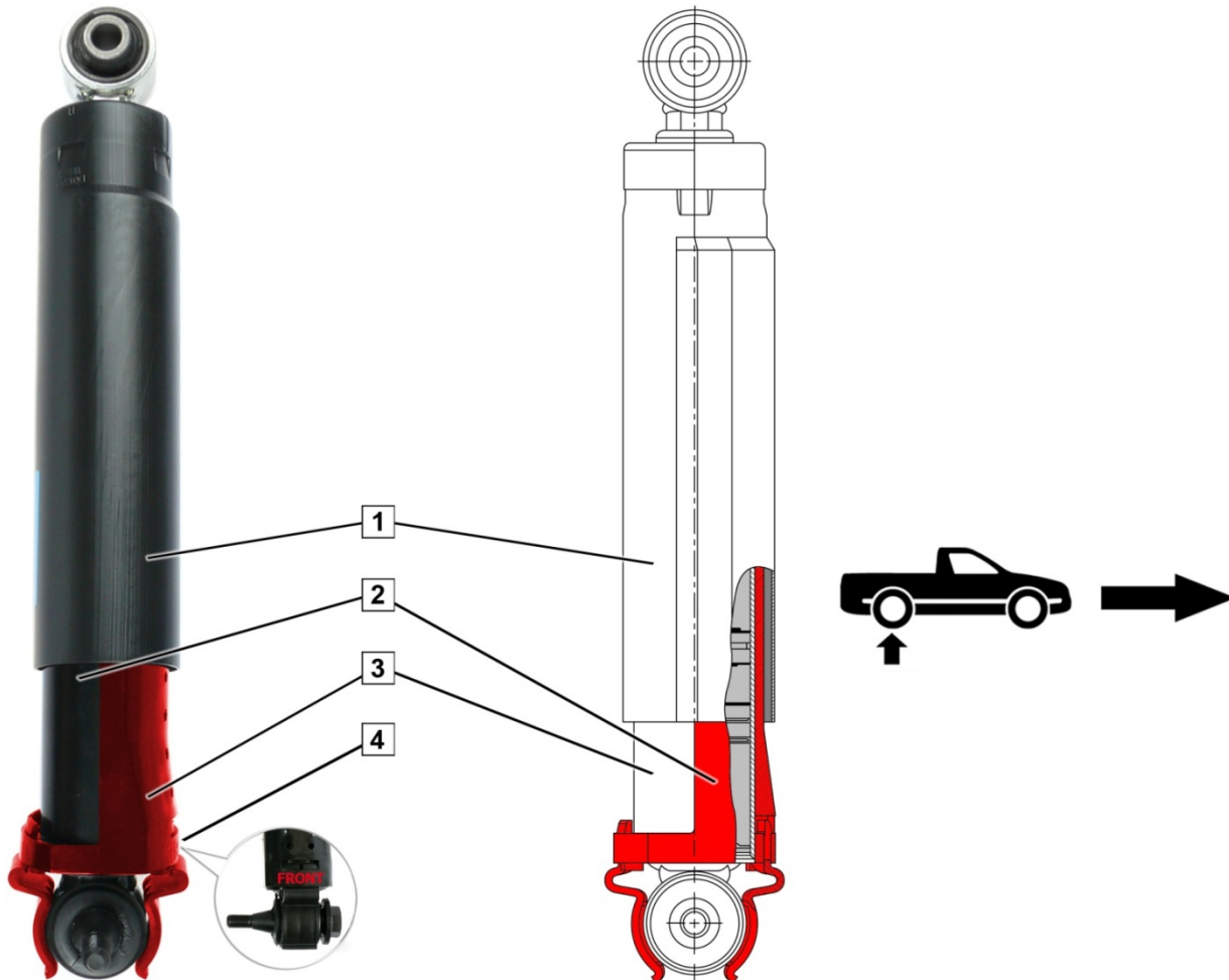
Fig. 1: Shock absorber with additional protection sleeve
