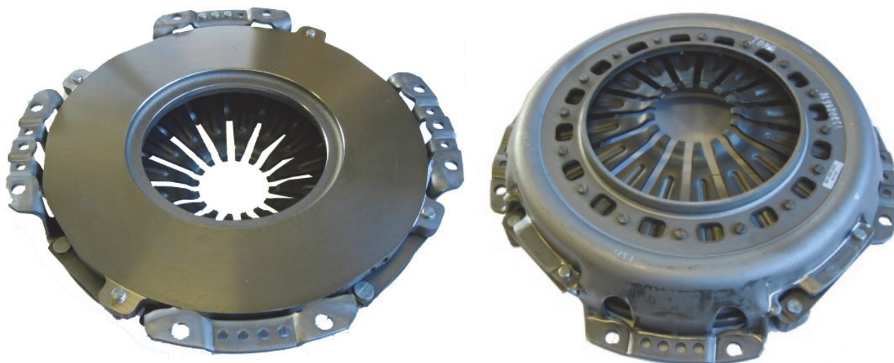
Fig. 1: 330 mm Single diaphragm-spring clutch
