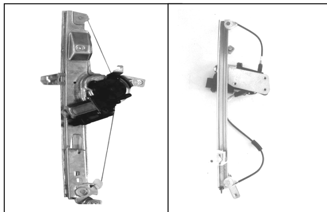
Elevavinas original – lève-vitre original – oem window regulator – levandator de vidro original
