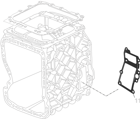
Side Housing Gasket
