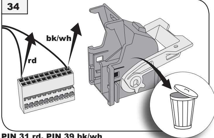
PIN 31 rd, PIN 39 bk/wh
