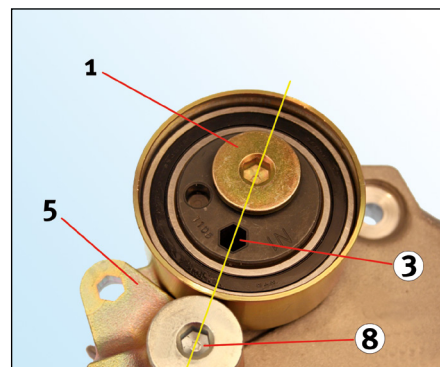
Figur 6: Forkert monteringsposition (set forfra)
