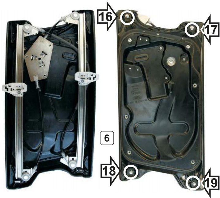
POWER WINDOW LEFT
