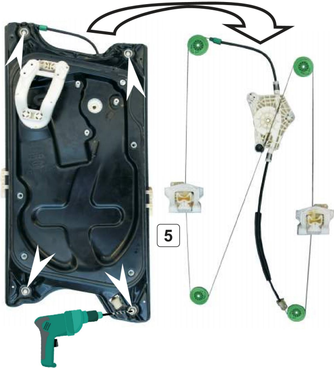
POWER WINDOW LEFT ORIGINAL
