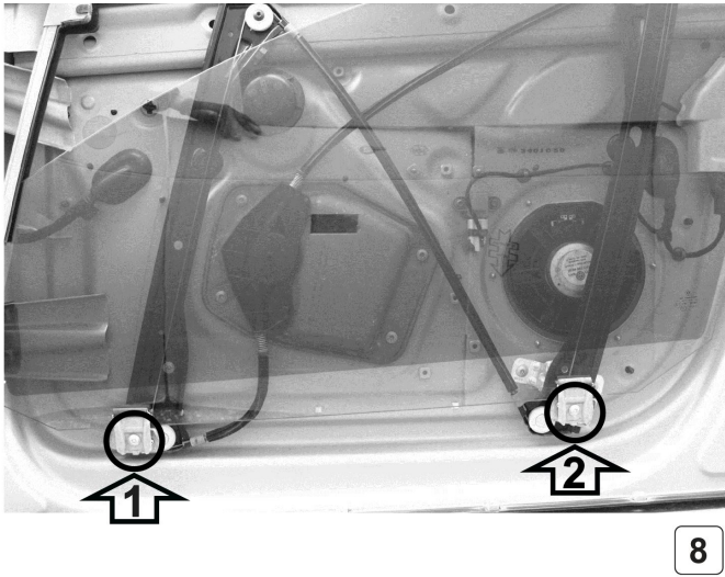
POWER WINDOW LEFT ORIGINAL
