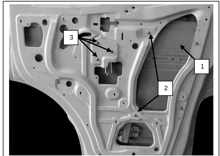
Porta lato sinistro, Portière avant gauche, Left front door, Puerta lado izquierdo, Vorne links Tür, Porta frente esquerda, Sol on kapı, πόρτα εμπρός/αριστερή
