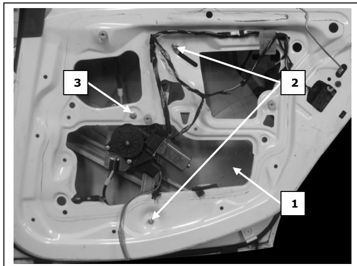
Porta lato destro, Portière arrière droite, Right rear door, Puerta lado derecho, Hinten rechte Tür, Porta traseira dirieta, Sag arka kapi, πόρτα οπίσθια δεξιά
