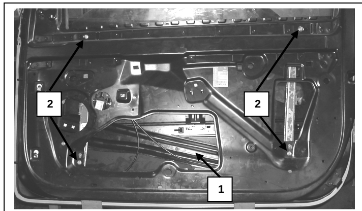
Porta lato destro, Portière avant droite, Right front door, Puerta lado derecho, Vorne rechte Tür, Porta frente dijeta, Sag on kapi, πόρτα εμπρόςδεξιά
