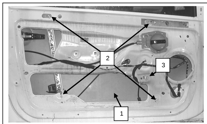
Porta lato sinistro, Portière avant gauche, Left front door, Puerta lado izquierdo, Vorne links Tür, Porta frente esquerda, Sol on kapı, πόρτα εμπρός/αριστερή
