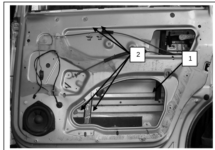
Porta lato destro, Portière arrière droite, Right rear door, Puerta lado derecho, Hinten rechte Tür, Porta traseira direita, Sag arka kapi, νότια οπίσθια δεξιά
