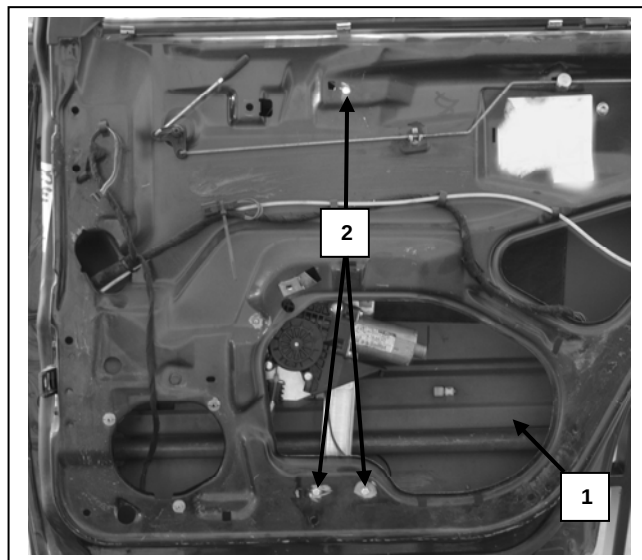
Porta lato destro, Portière arrière droite, Right rear door, Puerta lado derecho, Hinten rechte Tür, Porta traseira direita, Sag arka kapi, πόρτα οπίσθια δεξιά
