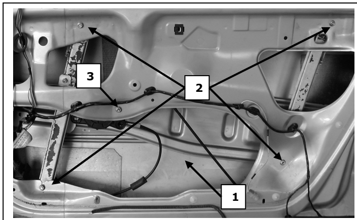
Porta lato destro, Portière avant droite, Right front door, Puerta lado derecho, Vorne rechte Tür, Porta frente dirieta, Sag on kapı, πόρτα εμπρός/δεξιά
