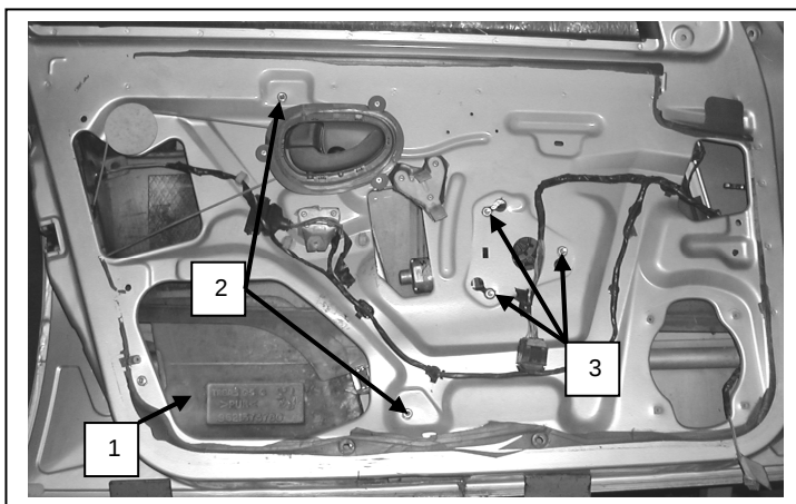
Porta lato sinistro, Portière avant gauche, Left front door, Puerta lado izquierdo, Vorne links Tür, Porta frente esquerda, Sol on kapı, πόρτα εμπρόσθια αριστερή
