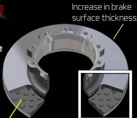
Pillar vent design creating significantly more airflow.
