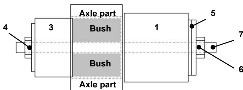
Tool installed; bush dismantling begins
