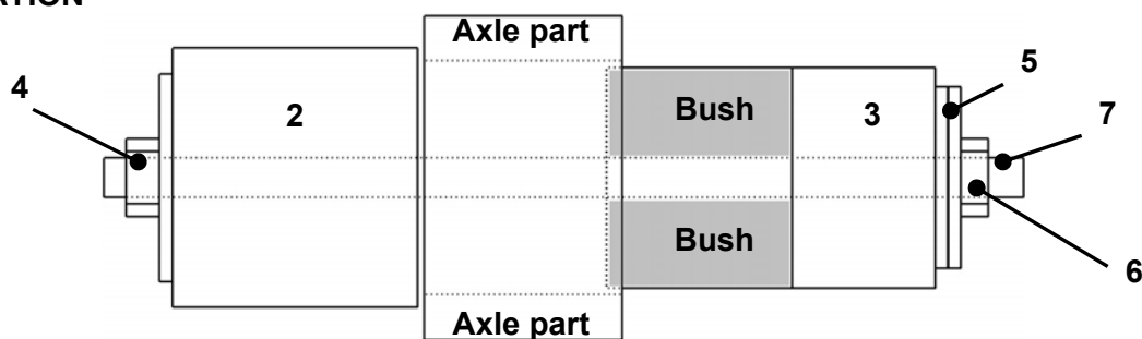
Tool installed; bush mounting begins
